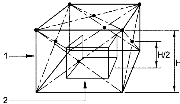
FIG. 324 Microphone Positions for All Other Hand-Held Toys
