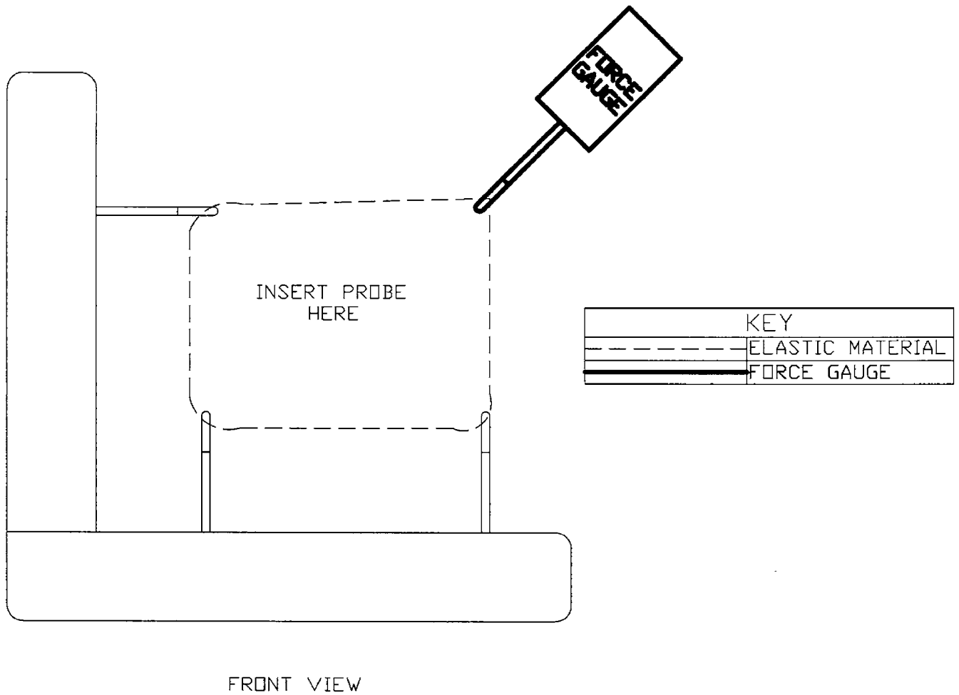
FIG. 346 (e) Test Procedure for Cords and Loops, Step 5 (continued)
