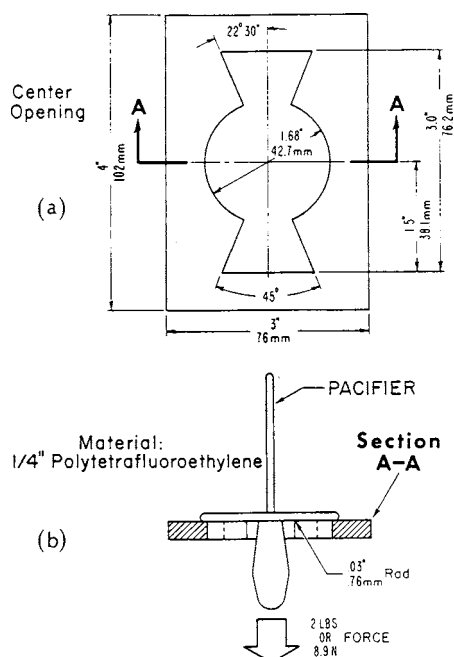
FIG. 154 Pacifier Test Fixture
