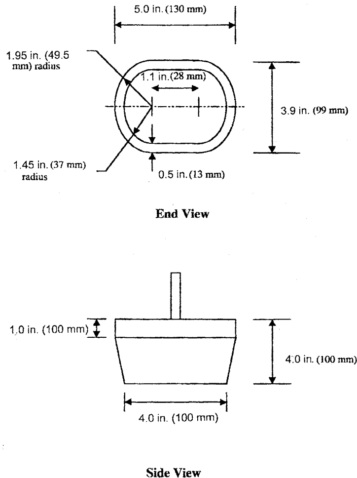
FIG. 110 Head Probe for Cords and Elastics
