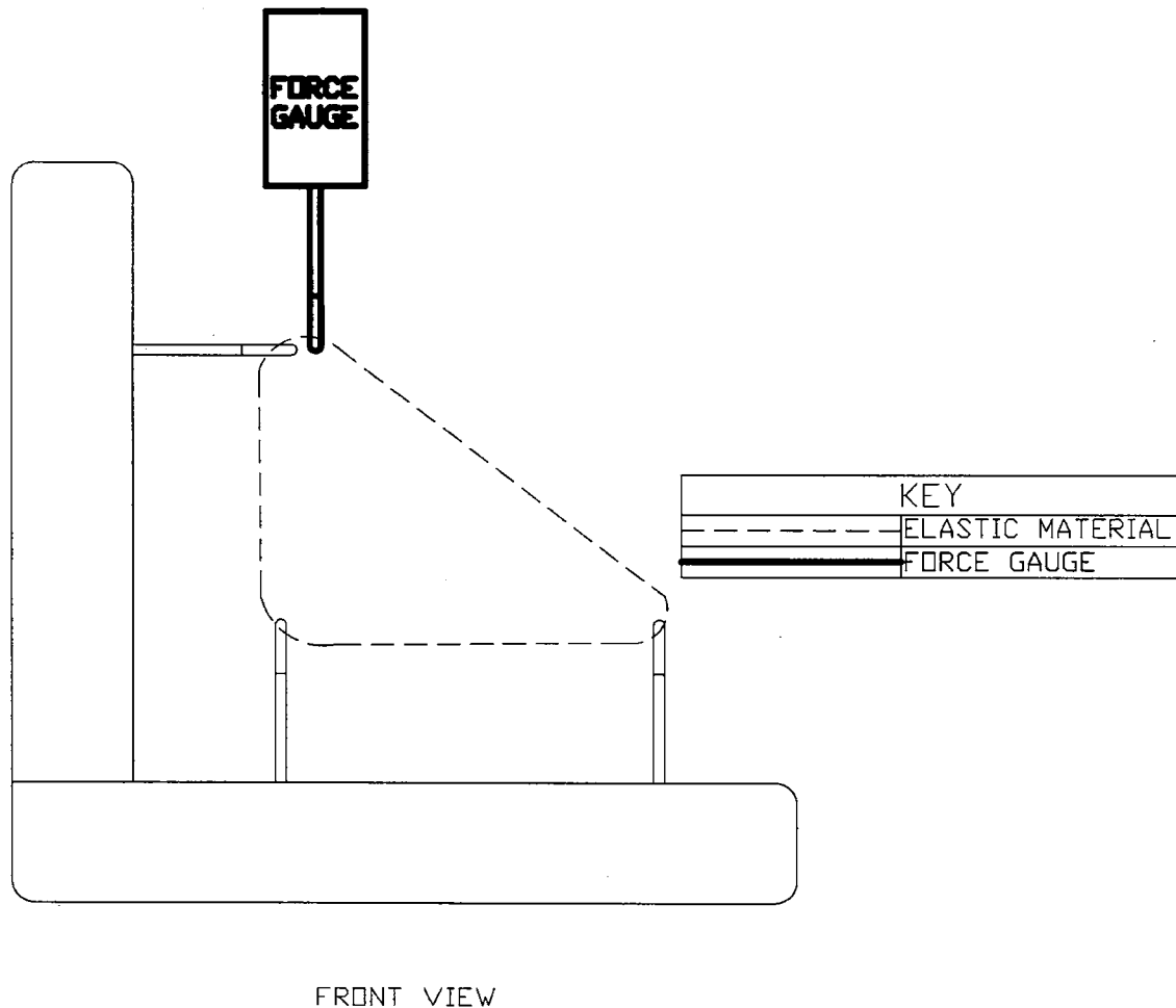
FIG. 346 (c) Test Procedure for Cords and Loops, Step 3 (continued)
