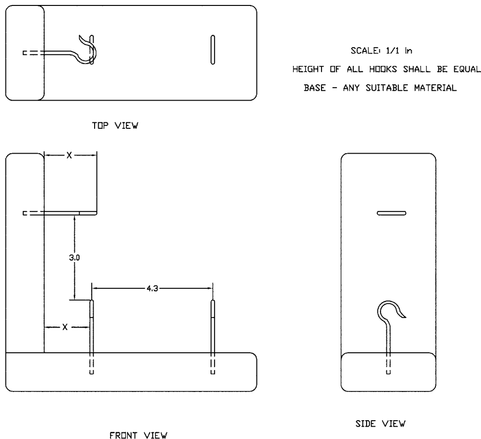
FIG. 346 Hook Test Fixture for Cords and Loops
