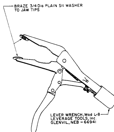
FIG. 257 Seam Clamp
