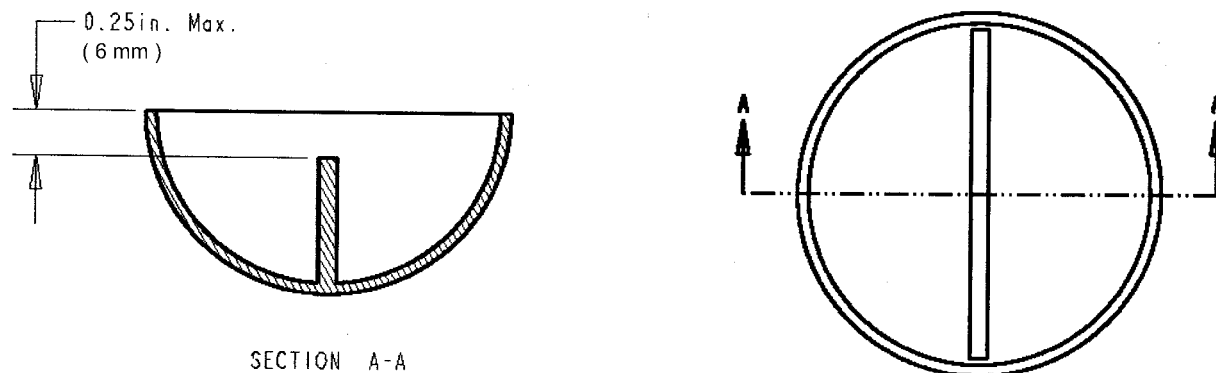
FIG. 223 Rib Through Cup Center
