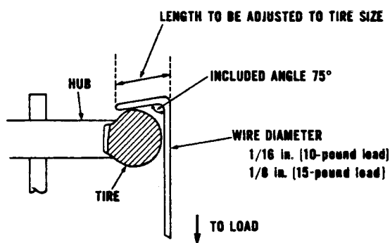
FIG. 268 Hook for Tire Removal
