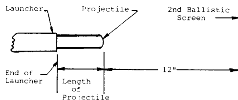
FIG.-29 31 Diagram of Layout to Determine Projectile Velocity
