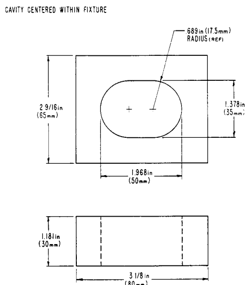
FIG. 165 Rattle Test Fixture
