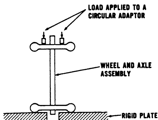
FIG. 279 Compression Test for Wheel Assemblies
