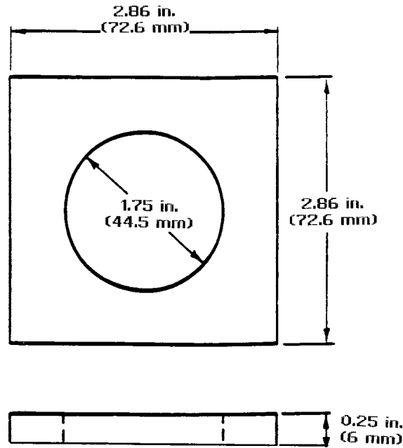
FIG. 19 20 Test Fixture for Small Balls
