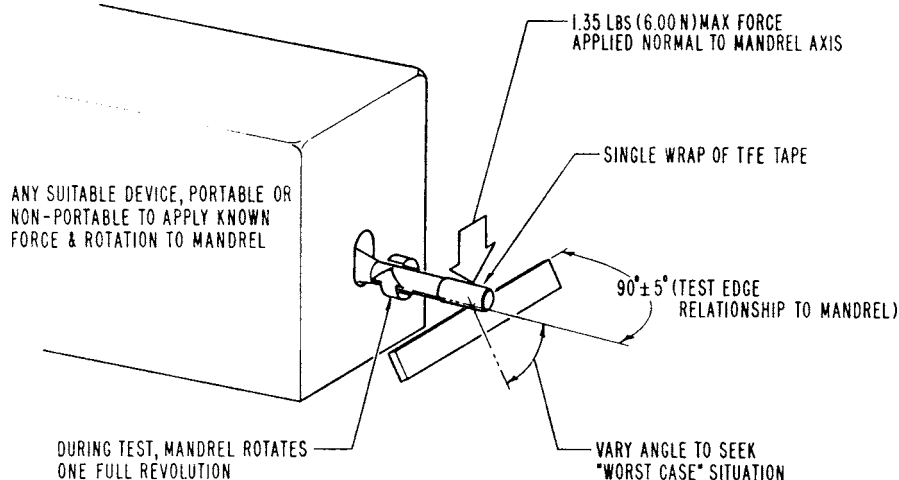
FIG. 9 Principle of Sharp Edge Test
