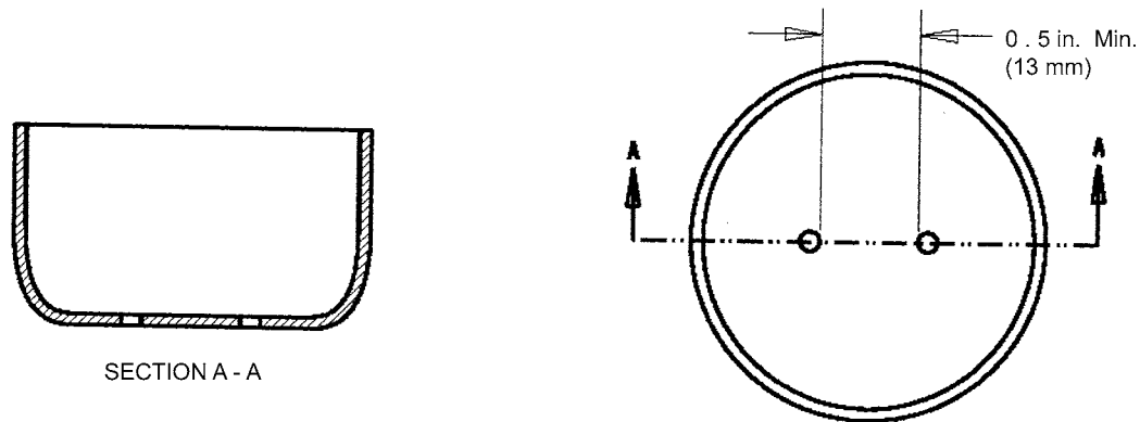
FIG. 201 Openings in Base of Bowl
