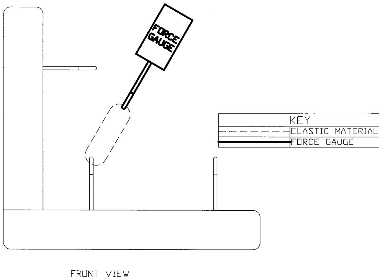
FIG. 346 (a) Test Procedure for Cords and Loops, Step 1 (continued)
