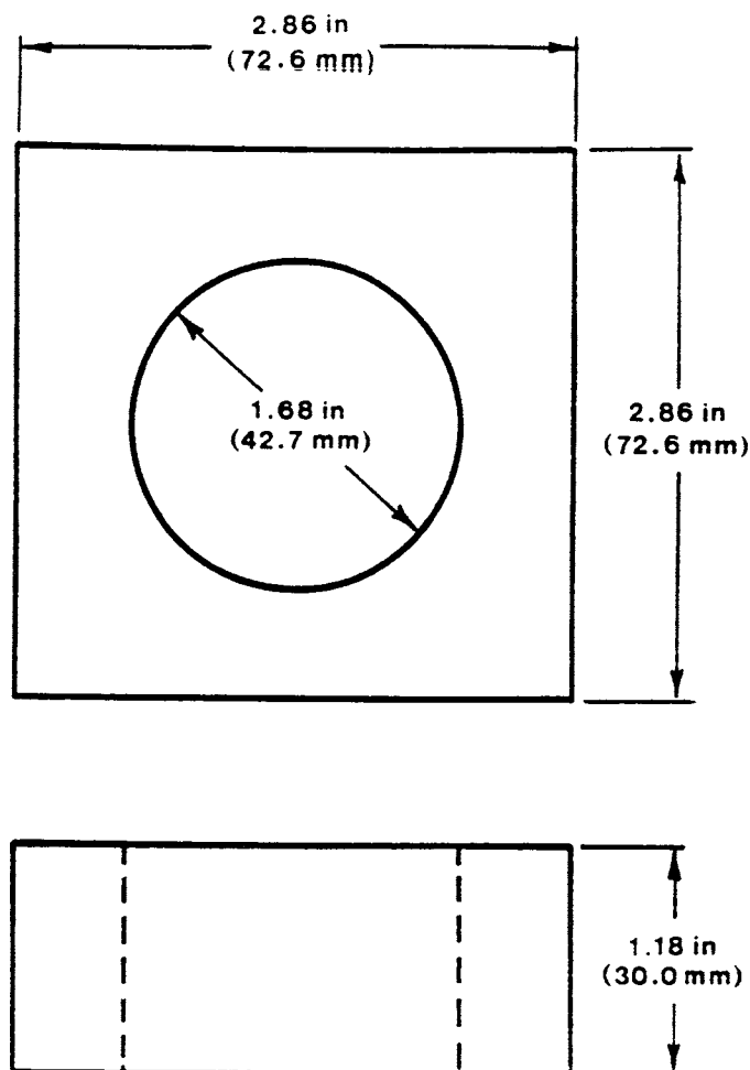
FIG. 176 Supplemental Test Fixture for Rattles, Squeeze Toys, and Teethers
